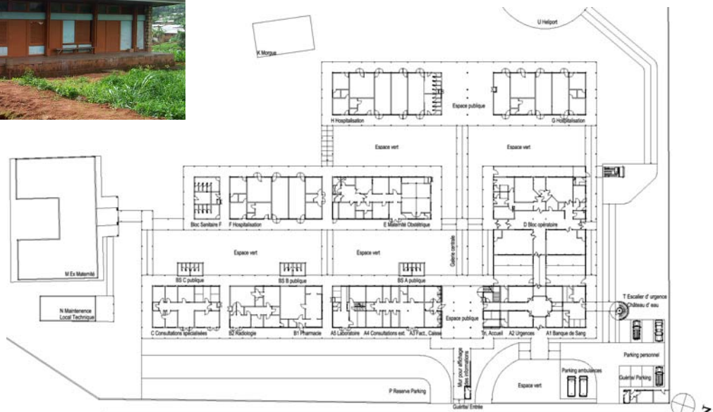
District Hospital Edia, ground plan
